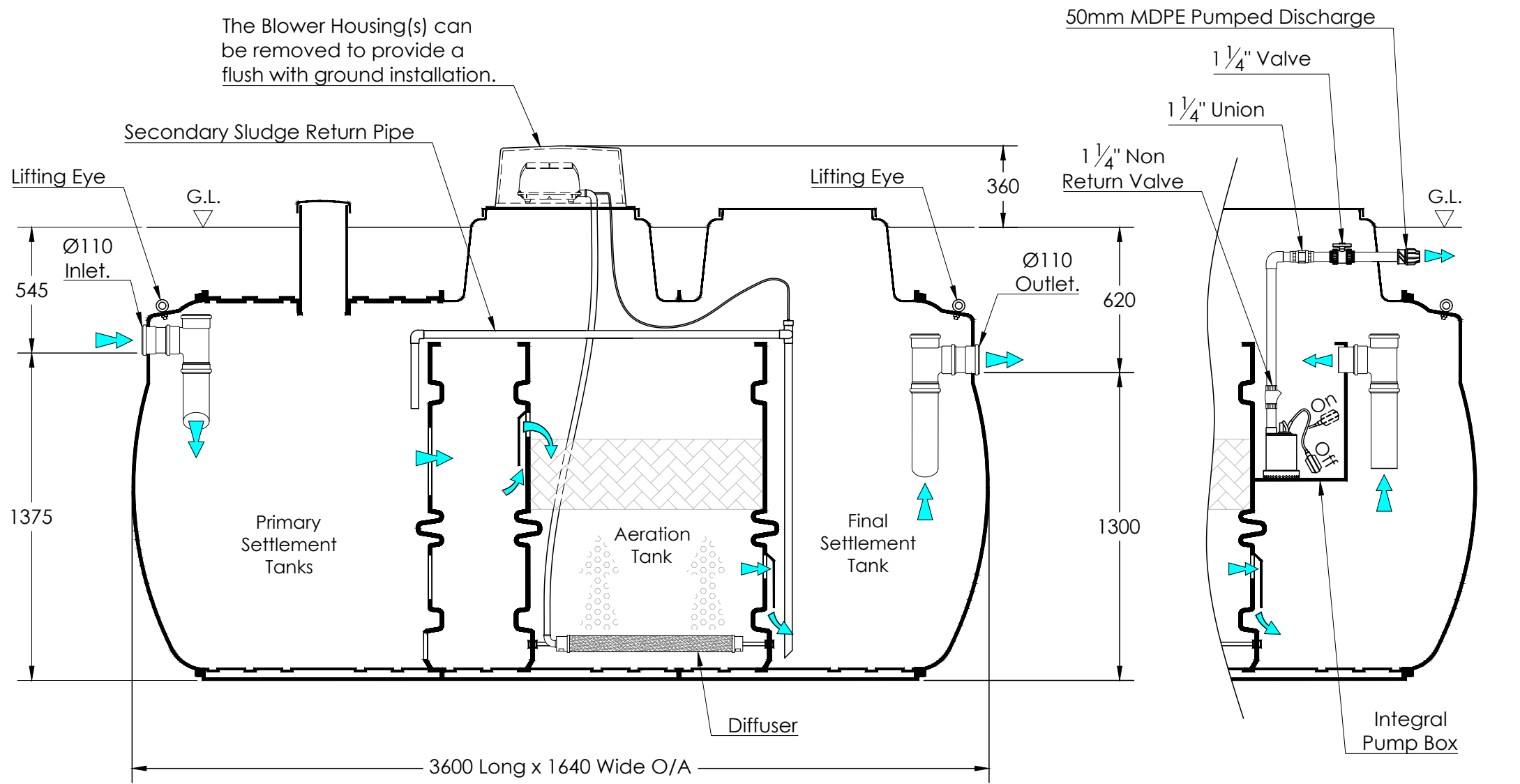
VERTICAL SECTION ON C-C
