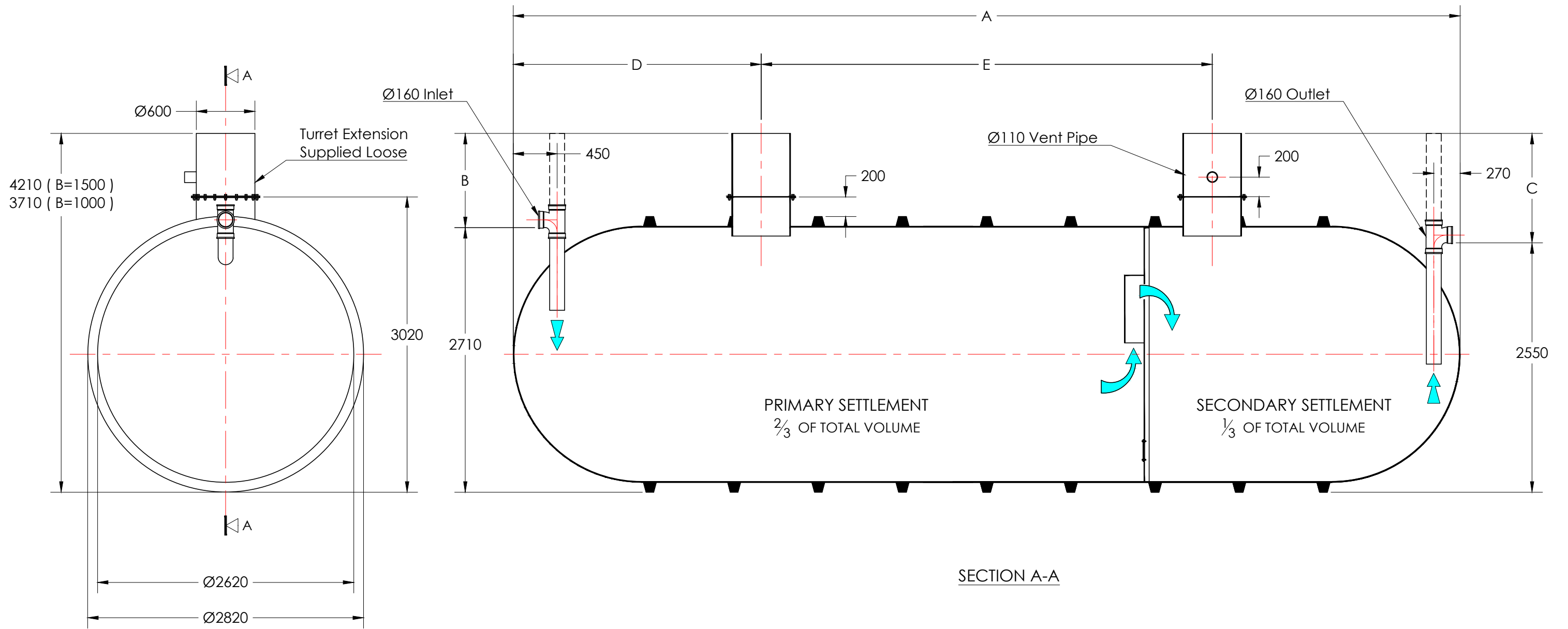
FRONT ELEVATION
