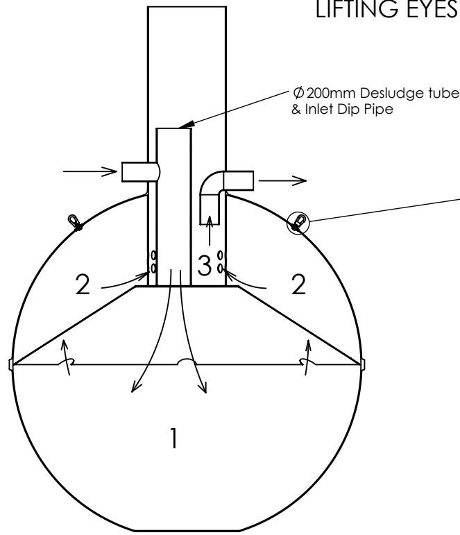
SECTION VIEW
