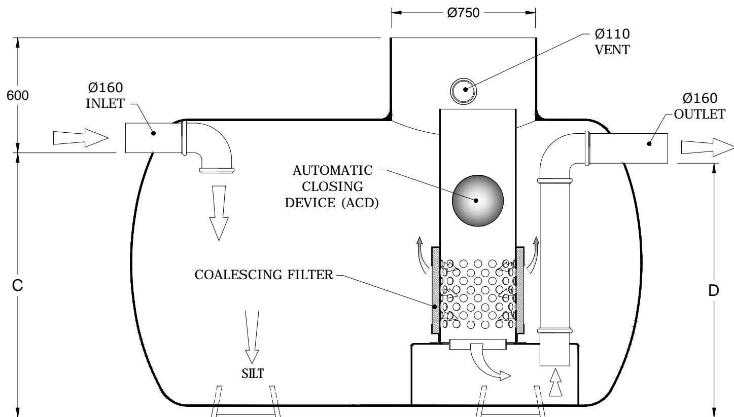
PART SECTION VIEW X-X
