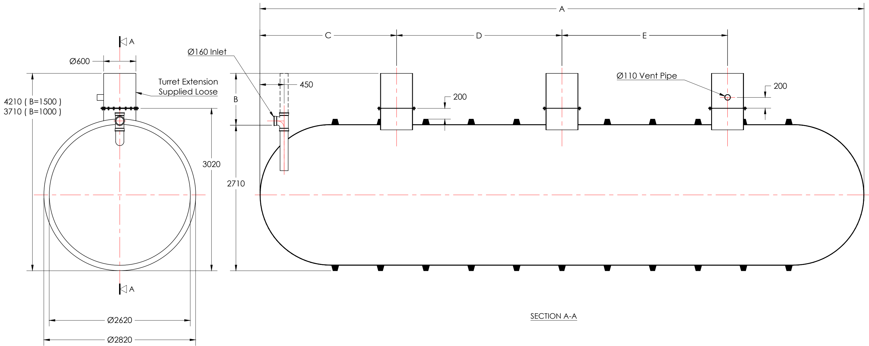
FRONT ELEVATION
