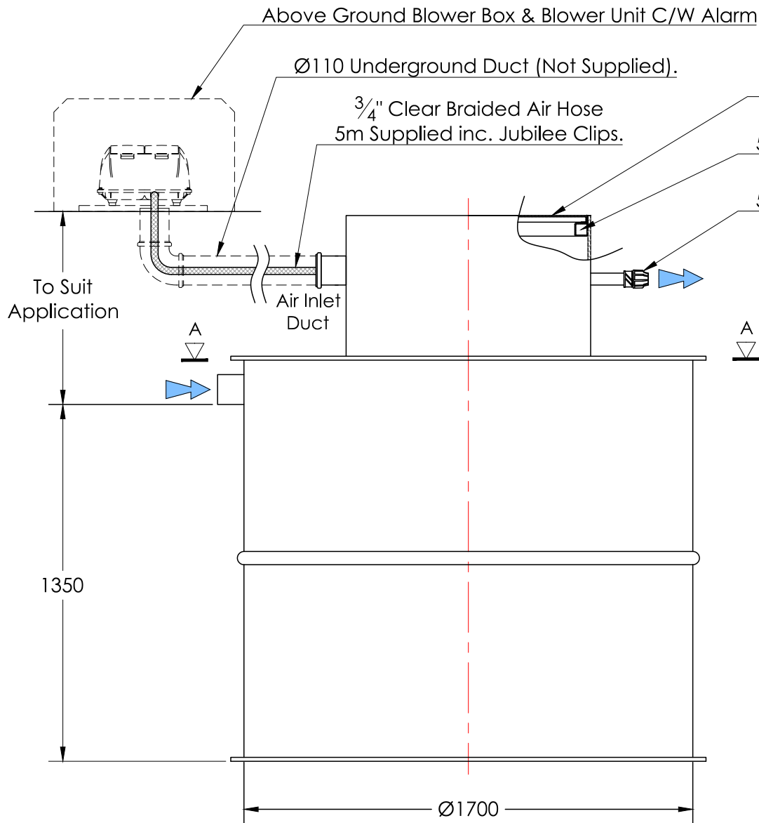
FRONT ELEVATION
